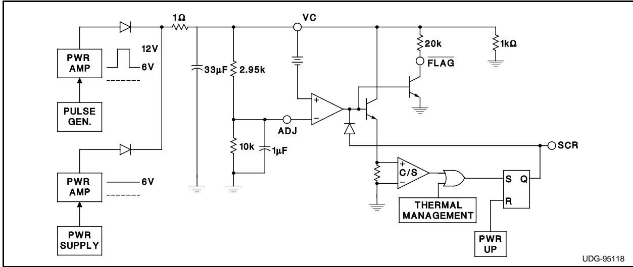
Figure 3. Lab Evaluation Circuit
